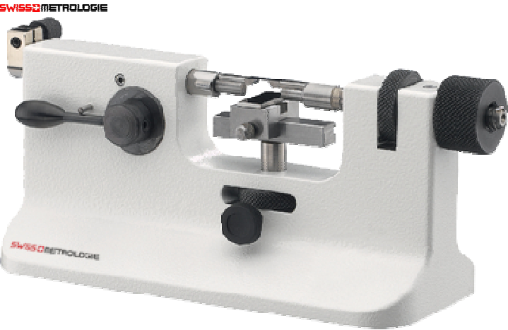
MONO-BLOCK STRUCTURE
